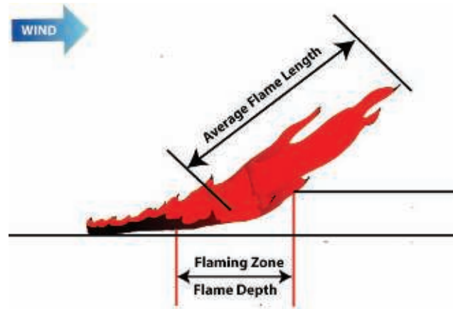
Flame dimensions for a wind driven fire.
